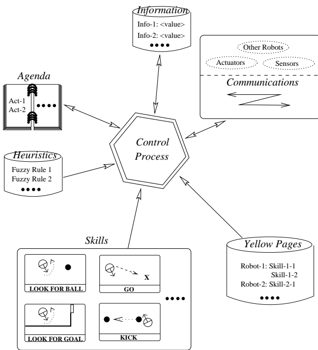
Figure 1: Architecture of the Robots.
